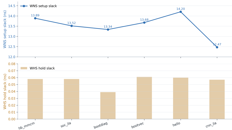
Figure 4.9: Timing closure summary across diagnostic and CNN board build configurations; all recorded builds meet setup and hold timing with positive slack.
