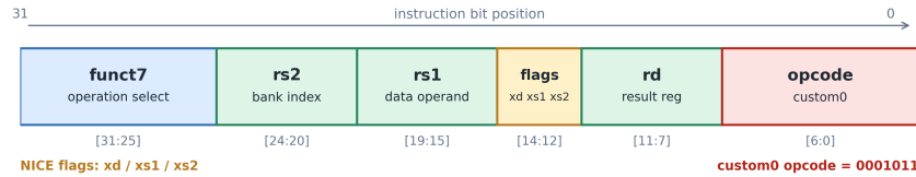
Figure 3.2: RISC-V custom0 instruction format used by the accelerator; bits [14:12] carry the NICE xd/xs1/xs2 flags and funct7 selects the accelerator operation.
