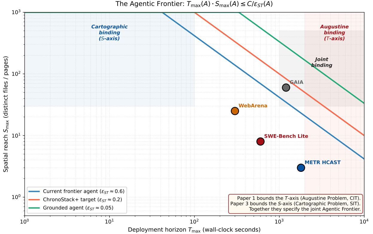
Figure 8: The Agentic Frontier in the (T, S) plane. Each curve is a level set T \cdot S = C/\varepsilon_{ST}(A) for one value of the spatiotemporal calibration error. Major long-horizon agent benchmarks are placed at their characteristic temporal and spatial load. Paper 1 bounds the temporal ( T ) axis through the Augustine Problem and CIT; Paper 3 extends to the spatial ( S ) axis through the Cartographic Problem and SIT; together they specify the joint frontier.
