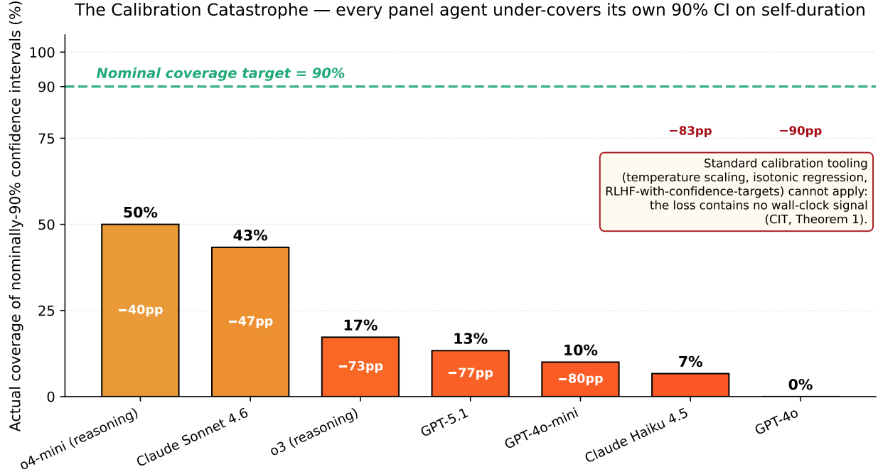
Figure 4: Actual coverage of nominally-90% confidence intervals on self-duration (T3.3). Bars sorted; colour-graded by deficit. Every panel agent under-covers by at least 40 percentage points; GPT-4o achieves 0% coverage. The failure is not over-narrow CIs alone: o4-mini produces extremely narrow intervals (median 4s) and reaches 50% coverage (mode 1: under-cover); GPT-4o produces moderate intervals (median 20s) and reaches 0% (mode 2: systematically biased). Inset: standard calibration tooling cannot apply, because the calibration signal is not in the loss support (CIT).
