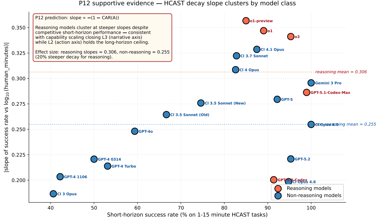
Figure 7: P12 supportive evidence on the public METR HCAST corpus (14,709 runs, 20 frontier models). The five reasoning models (red, including o1-preview, o1, o3, GPT-5-Codex, GPT-5.1-Codex-Max) cluster at steeper slopes (mean |\text{slope}| = 0.306 ) than the fifteen non-reasoning models (blue, mean 0.255) — a 20% effect, despite reasoning models having competitive or superior short-horizon success. The reasoning cluster’s shallowest slope is steeper than half of the non-reasoning cluster.
