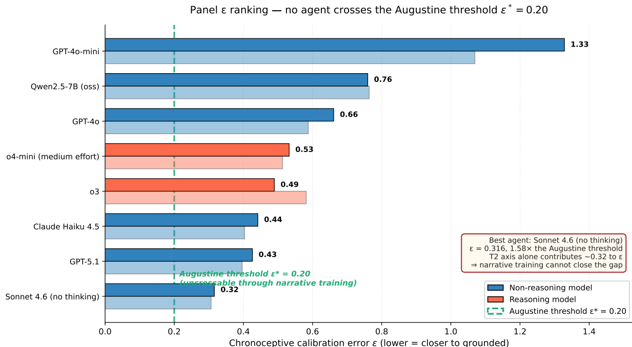
Figure 6: Panel \epsilon ranking. Setting A bars sorted; Setting B bars (lighter) below. The dashed green line marks \epsilon^* = 0.20 . No agent crosses the threshold. The best agent (Sonnet 4.6 without thinking, \epsilon = 0.316 ) sits 1.58\times above; its T2 axis alone contributes \approx 0.32 , irreducible by any narrative-axis intervention. The Reverse-Scaling variants of o4-mini and Sonnet 4.6 are not shown here (Figure 3 carries their effect); the full sub-capability decomposition is in Appendix D.
