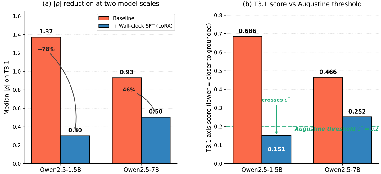
Toy positive control: wall-clock SFT reduces |\rho| at both scales; 1.5B crosses \varepsilon^* on T3.1, 7B falls short
