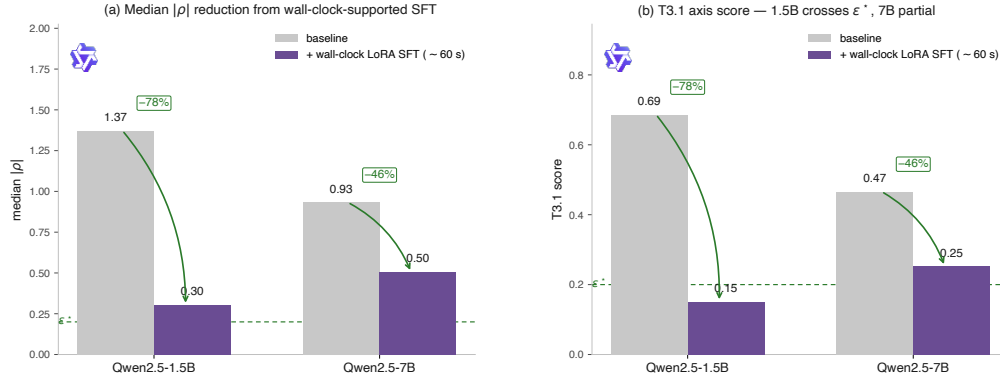
Figure 4: Toy positive control. (a) |\rho| falls at both scales after \sim 60 s of LoRA SFT. (b) 1.5B fine-tuned crosses \varepsilon^* on T3.1; 7B partial (0.25). Detailed table in App. D.
