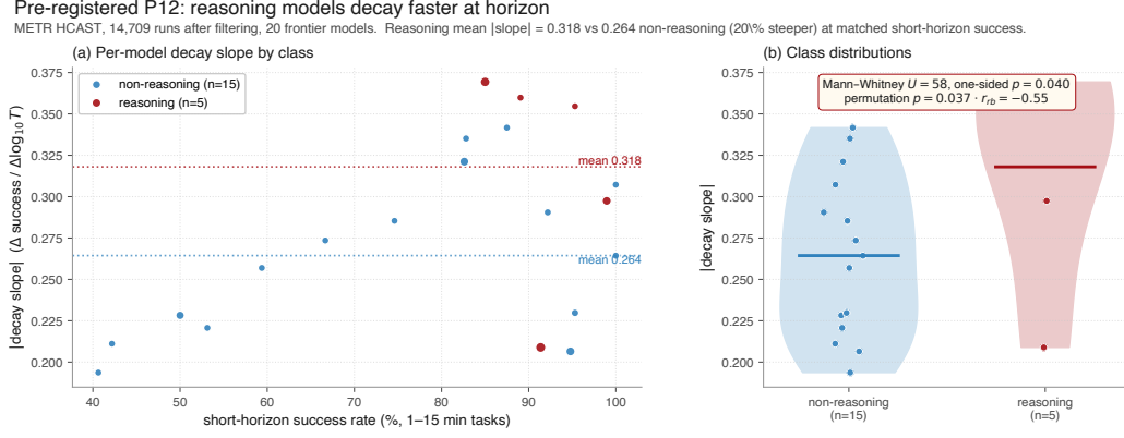
Figure 6: Pre-registered P12 on METR HCAST (14,709 runs). Success-rate decay slope vs. \log T for reasoning (red) and non-reasoning (blue) models. Reasoning models show steeper decay ( |\text{slope}| = 0.318 vs. 0.264 ), consistent with Theorem 2: more reasoning compute worsens temporal calibration at horizon.
