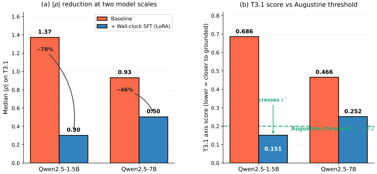
Toy positive control: wall-clock SFT reduces |\rho| at both scales; 1.5B crosses \varepsilon^* on T3.1, 7B falls short
