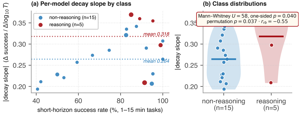
Figure 6: P12 support on METR HCAST. Reasoning models cluster at steeper decay slopes despite competitive short-horizon success — the L2 mechanism at the model-class level.
