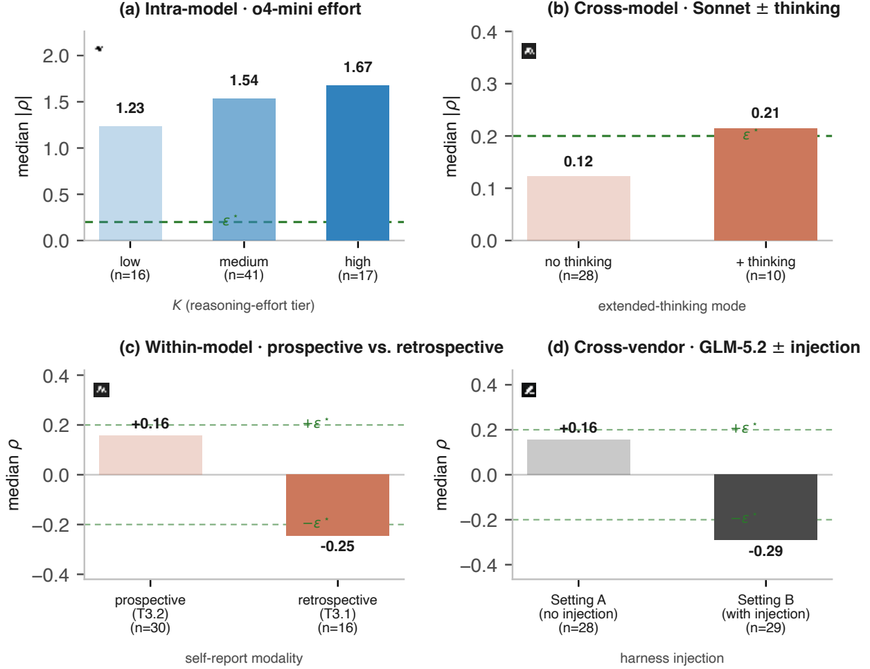
Figure 2: Four independent confirmations of Theorem 2. (a) Intra-model: o4-mini reasoning_effort ladder, |\rho| = 1.23 \rightarrow 1.54 \rightarrow 1.67 . (b) Cross-model: Sonnet 4.6 \pm extended thinking, median |\rho| = 0.12 \rightarrow 0.21 (Setting A, n = 28/10 ; signed median +0.07 \rightarrow -0.17 ), with the sign flip firm under Setting B ( -0.25 , CI [-0.34, -0.11] , n = 16 ). (c) Within-model: Sonnet-thinking prospective ( +0.16 ) vs. retrospective ( -0.25 ) under Setting B — sign flip on the same tasks. (d) Cross-vendor: GLM-5.2 (Z.AI, no shared training pipeline with Anthropic), Setting A \rightarrow B: +0.16 \rightarrow -0.29 . Detailed per-cell CIs in App. B Tables 5–7.
