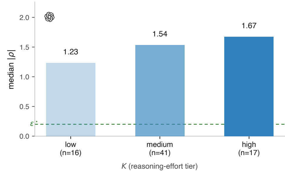
(a) Intra-model · o4-mini effort ladder
