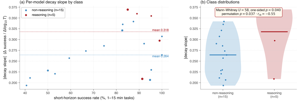
Figure 6: P12 support on METR HCAST. Reasoning models cluster at steeper decay slopes despite competitive short-horizon success — the L2 mechanism at the model-class level.
