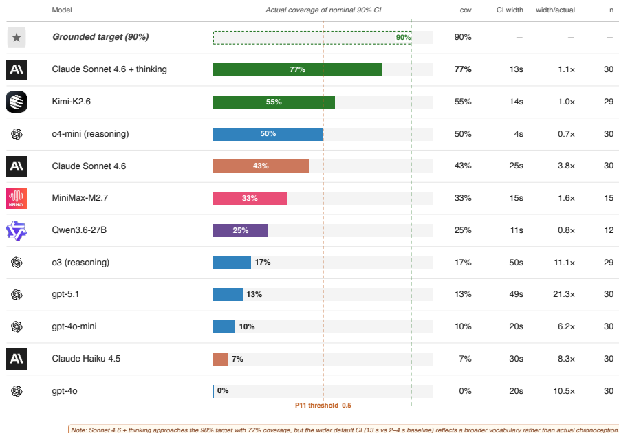
Figure 3: Actual coverage of nominally-90% CIs on self-duration (T3.3), 12-row panel. Only reasoning-mode agents (Sonnet + thinking, Kimi-K2.6) exceed the P11 threshold of 0.5 — both accidentally, through wider default vocabulary intersecting thinking-inflated \tau_{\text{wall}} (see App. D), not through learned chronoception.
