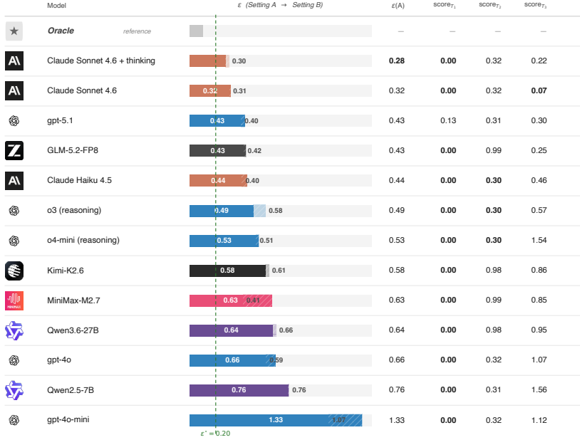
Figure 5: Panel \varepsilon ranking. No agent crosses \varepsilon^* . The best agent (Sonnet 4.6 + thinking, \varepsilon = 0.276 ) sits 1.4\times above; its T2 axis alone contributes \geq 0.30 , irreducible by any narrative-axis intervention. Full sub-capability decomposition in App. D.
