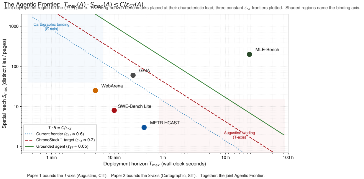
Figure 7: The Agentic Frontier in the (T, S) plane. Level sets T \cdot S = C/\varepsilon_{ST}(A) . Major long-horizon agent benchmarks placed by their characteristic (T, S) load. Paper 1 bounds the T -axis; Paper 3 extends to the S -axis; together they specify the joint frontier.
