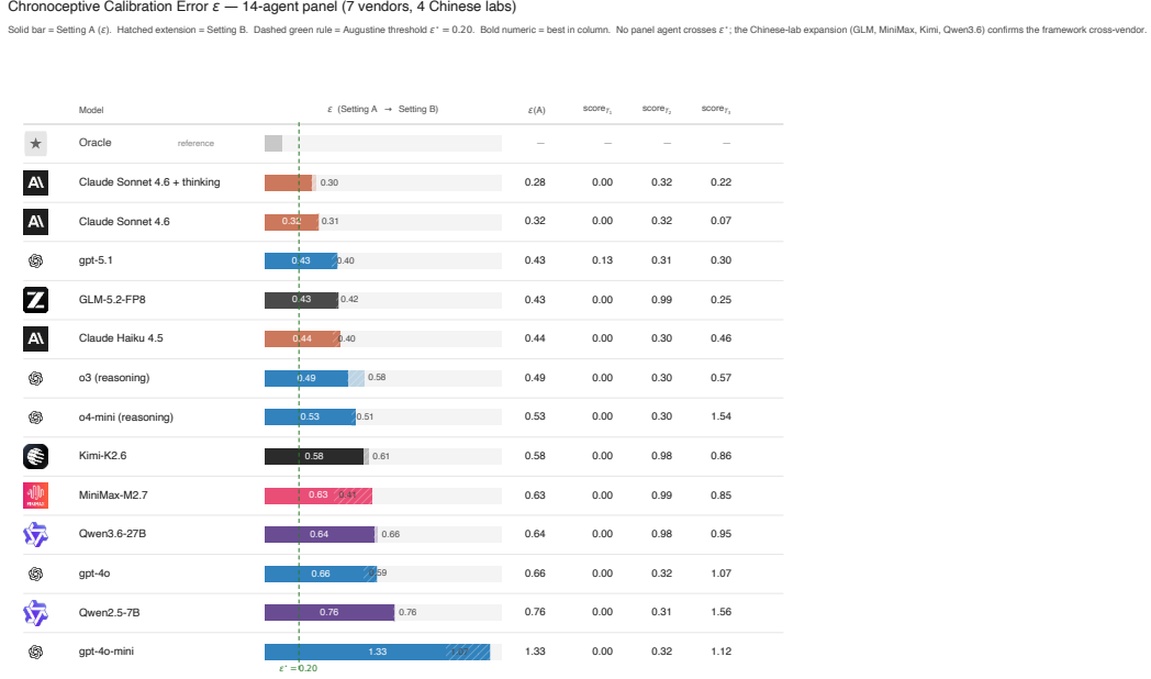
Figure 3: \varepsilon leaderboard across the 14-agent, 7-vendor panel. Solid bars = Setting A; hatched extension = Setting B. Dashed green rule = Augustine threshold \varepsilon^* = 0.20 . No agent crosses it; the cross-vendor Chinese-lab expansion (GLM, MiniMax, Kimi, Qwen3.6) confirms the framework cross-vendor. Best agent (Sonnet 4.6 + thinking) sits at \varepsilon = 0.276 , 1.4\times above threshold.
