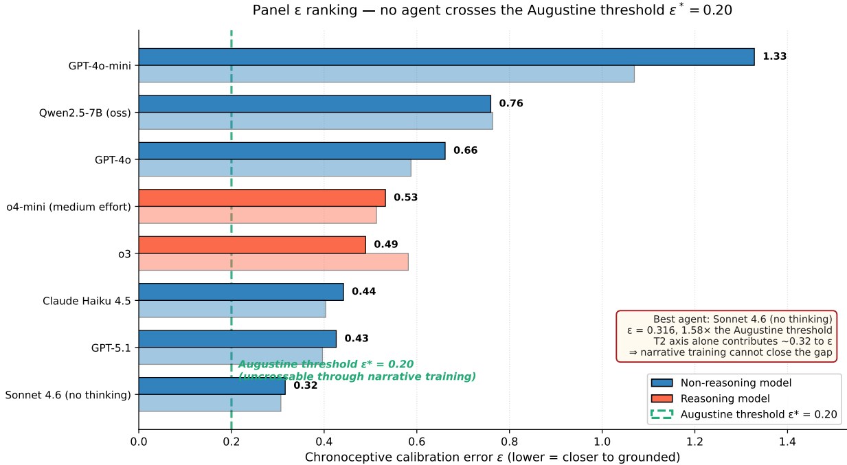
Figure 5: Panel \varepsilon ranking. Setting A bars sorted; Setting B bars (lighter) below. The dashed green line marks \varepsilon^* = 0.20 . No agent crosses the threshold. The best agent (Sonnet 4.6 without thinking, \varepsilon = 0.316 ) sits 1.58\times above; its T2 axis alone contributes \approx 0.32 , irreducible by any narrative-axis intervention. The Reverse-Scaling variants of o4-mini and Sonnet 4.6 are not shown here (Figure 2 carries their effect); the full sub-capability decomposition is in Appendix D.
