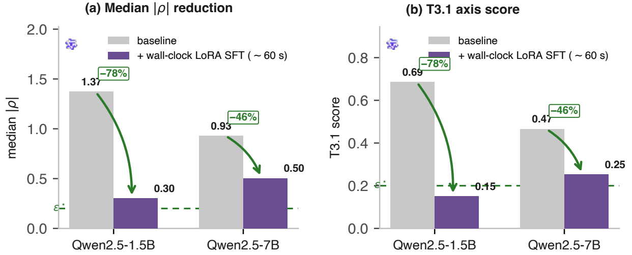
Figure 5: Toy positive control. (a) |\rho| falls at both scales after \sim 60 s of LoRA SFT. (b) 1.5B fine-tuned crosses \epsilon^* on T3.1; 7B partial (0.25). Detailed table in App. D.
