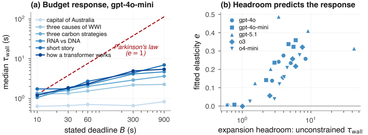
Figure 2: E11. (a) The budget response itself: median \tau_{\text{wall}} against the stated deadline, one line per question, against the diagonal Parkinson’s law would trace. (b) Why the lines differ: the fitted elasticity against the task’s expansion headroom, across five agents.
