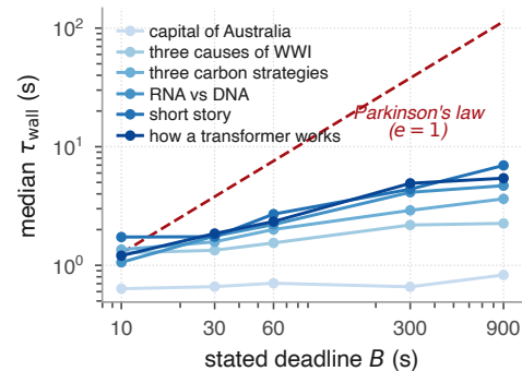
(a) Budget response, gpt-4o-mini
