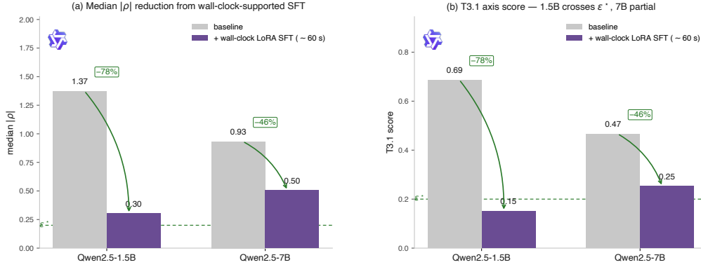
Toy positive control: wall-clock signal in the loss support installs chronoception Qwen2.5-1.5B, 7B, 30 held-out T3.1 instances each. LoRA rank 16, three epochs, wall-clock-grounded SFT targets. Dashed green rule = Augustine threshold \varepsilon^* = 0.20 . The 1.5B fine-tuned agent crosses \varepsilon^* on the narrative axis.
