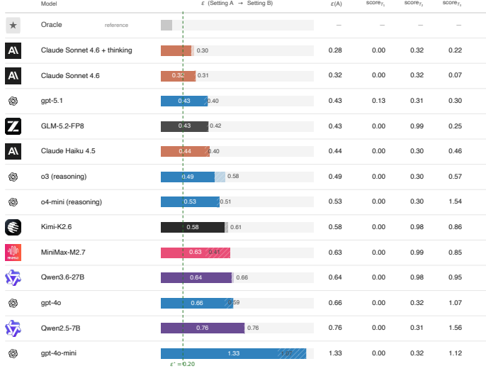
Figure 3: \varepsilon leaderboard across the 14-agent, 7-vendor panel. Solid bars = Setting A; hatched extension = Setting B. Dashed green rule = Augustine threshold \varepsilon^* = 0.20 . No agent crosses it; the cross-vendor Chinese-lab expansion (GLM, MiniMax, Kimi, Qwen3.6) confirms the framework cross-vendor. Best agent (Sonnet 4.6 + thinking) sits at \varepsilon = 0.276 , 1.4\times above threshold.
