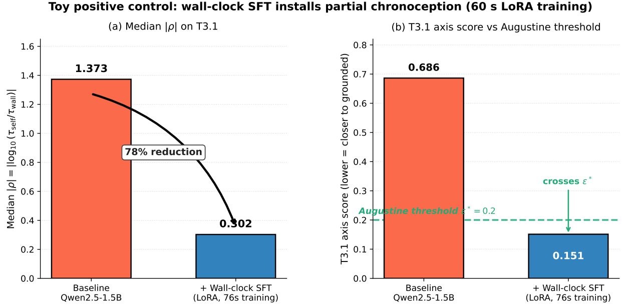
Figure 5: Toy positive control on T3.1. (a) Median |\rho| falls 78% after 76 seconds of LoRA fine-tuning with wall-clock-grounded SFT targets. (b) The fine-tuned model’s T3.1 axis score crosses the Augustine threshold \varepsilon^* = 0.20 ; the baseline does not. Each bar is the median over 30 held-out T3.1 instances.
