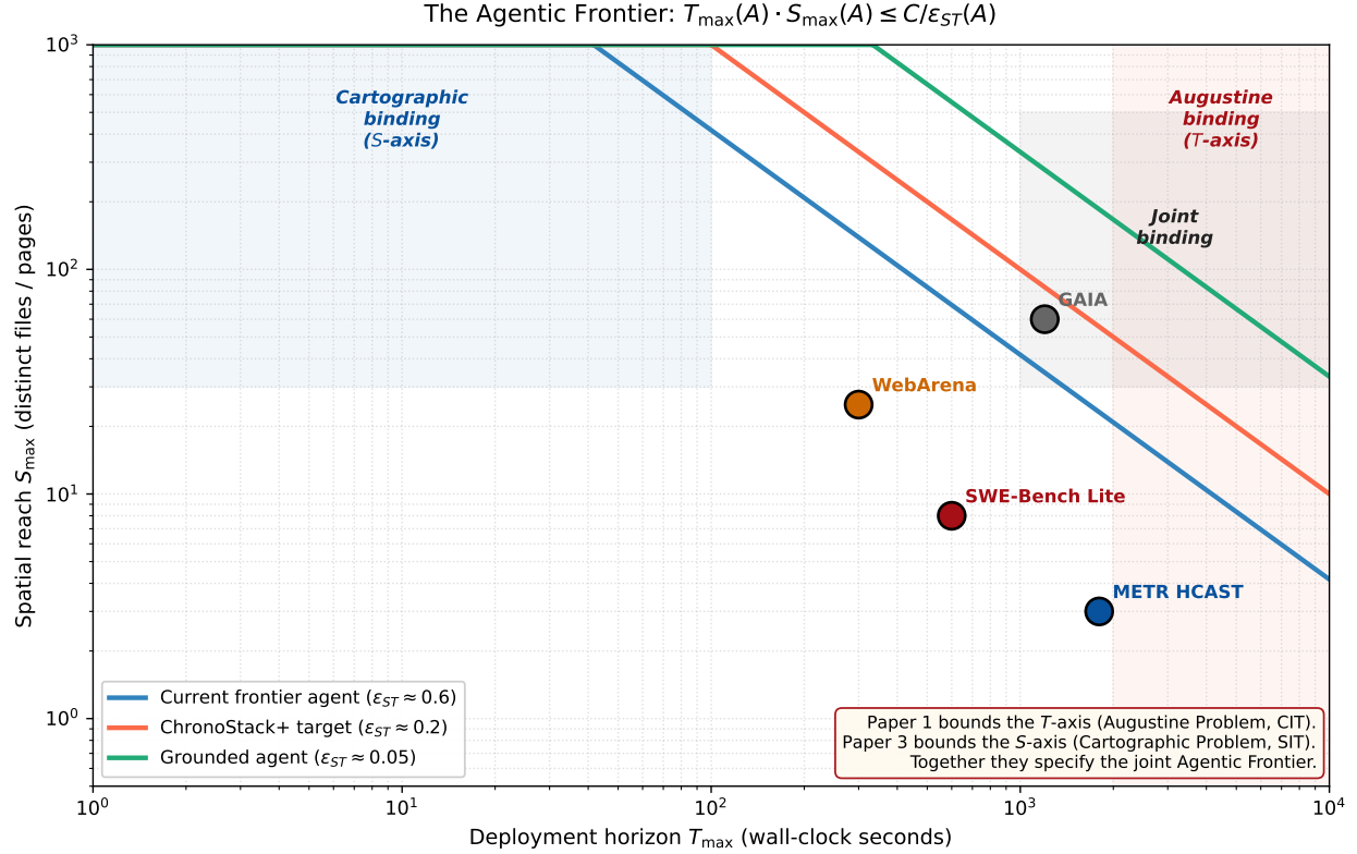
Figure 7: The Agentic Frontier in the (T, S) plane. Level sets T \cdot S = C/\varepsilon_{ST}(A) . Major long-horizon agent benchmarks placed by their characteristic (T, S) load. Paper 1 bounds the T -axis; Paper 3 extends to the S -axis; together they specify the joint frontier.
