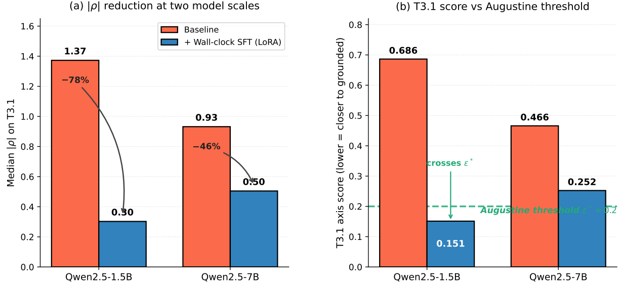
Figure 4: Toy positive control on T3.1 at two model scales. (a) Median |\rho| falls at both scales after \sim 60 s of LoRA fine-tuning with wall-clock-grounded SFT targets (78% reduction on Qwen2.5-1.5B; 46% on Qwen2.5-7B). (b) On the 1.5B model the fine-tuned T3.1 score crosses the Augustine threshold \varepsilon^* = 0.20 ; on the 7B model it falls short of the threshold (0.252). The direction is consistent at both scales; the magnitude of effect required to cross \varepsilon^* depends on base-model prior strength. Each bar is the median over 30 held-out T3.1 instances.
