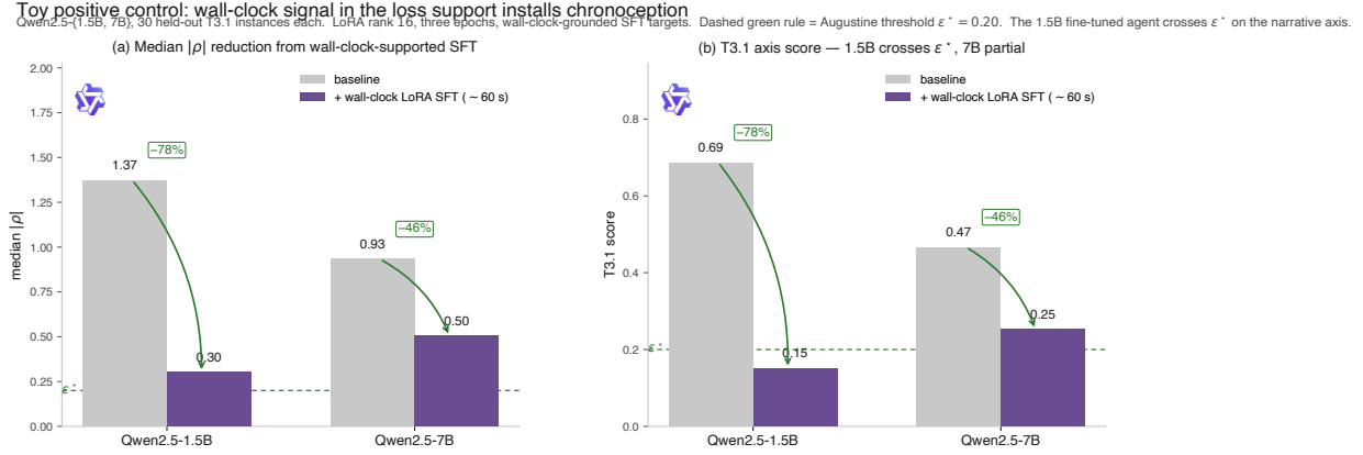
Figure 4: Toy positive control on T3.1 at two model scales. (a) Median |\rho| falls at both scales after \sim 60 s of LoRA fine-tuning with wall-clock-grounded SFT targets (78% reduction on Qwen2.5-1.5B; 46% on Qwen2.5-7B). (b) On the 1.5B model the fine-tuned T3.1 score crosses the Augustine threshold \varepsilon^* = 0.20 ; on the 7B model it falls short of the threshold (0.252). The direction is consistent at both scales; the magnitude of effect required to cross \varepsilon^* depends on base-model prior strength. Each bar is the median over 30 held-out T3.1 instances.
