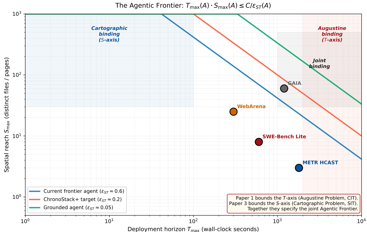
Figure 7: The Agentic Frontier in the (T, S) plane. Each curve is a level set T \cdot S = C/\varepsilon_{ST}(A) for one value of the spatiotemporal calibration error. Major long-horizon agent benchmarks are placed at their characteristic temporal and spatial load. Paper 1 bounds the temporal ( T ) axis through the Augustine Problem and CIT; Paper 3 extends to the spatial ( S ) axis through the Cartographic Problem and SIT; together they specify the joint frontier.
