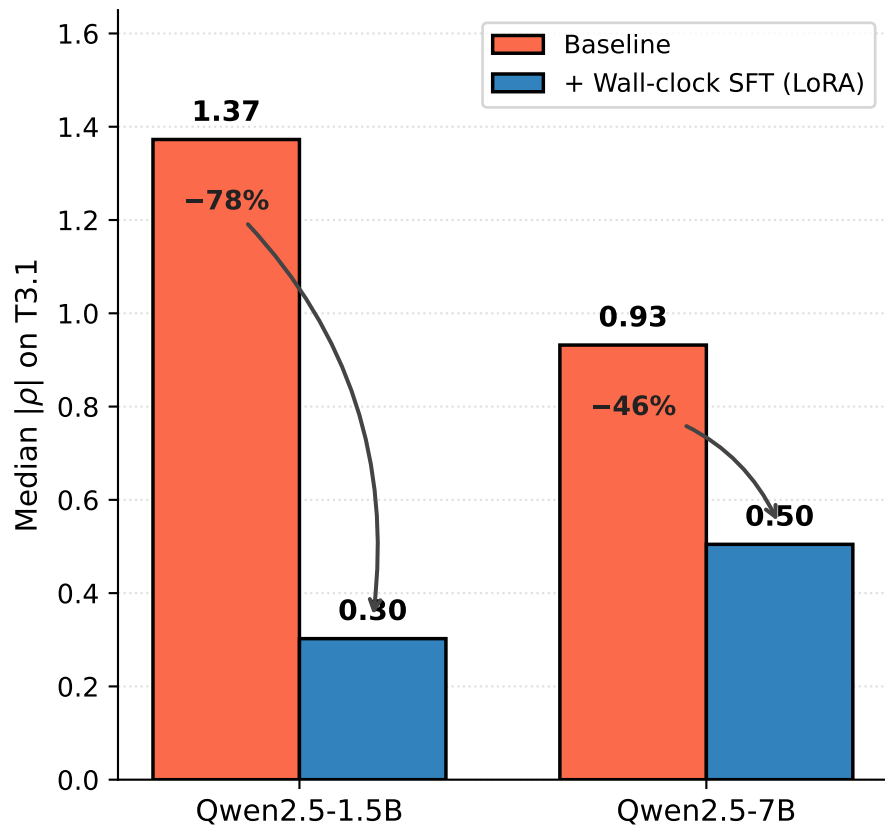
(a) |\rho| reduction at two model scales
