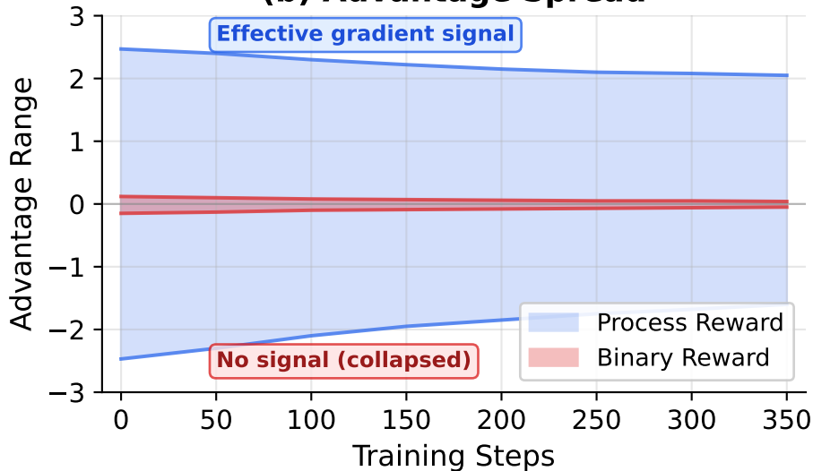
(b) Advantage Spread
