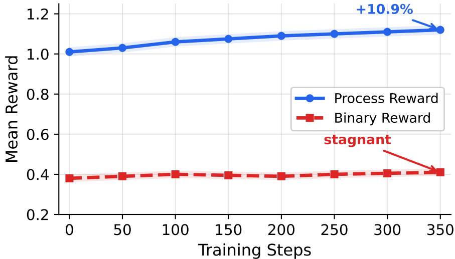
(a) Reward Trajectory
