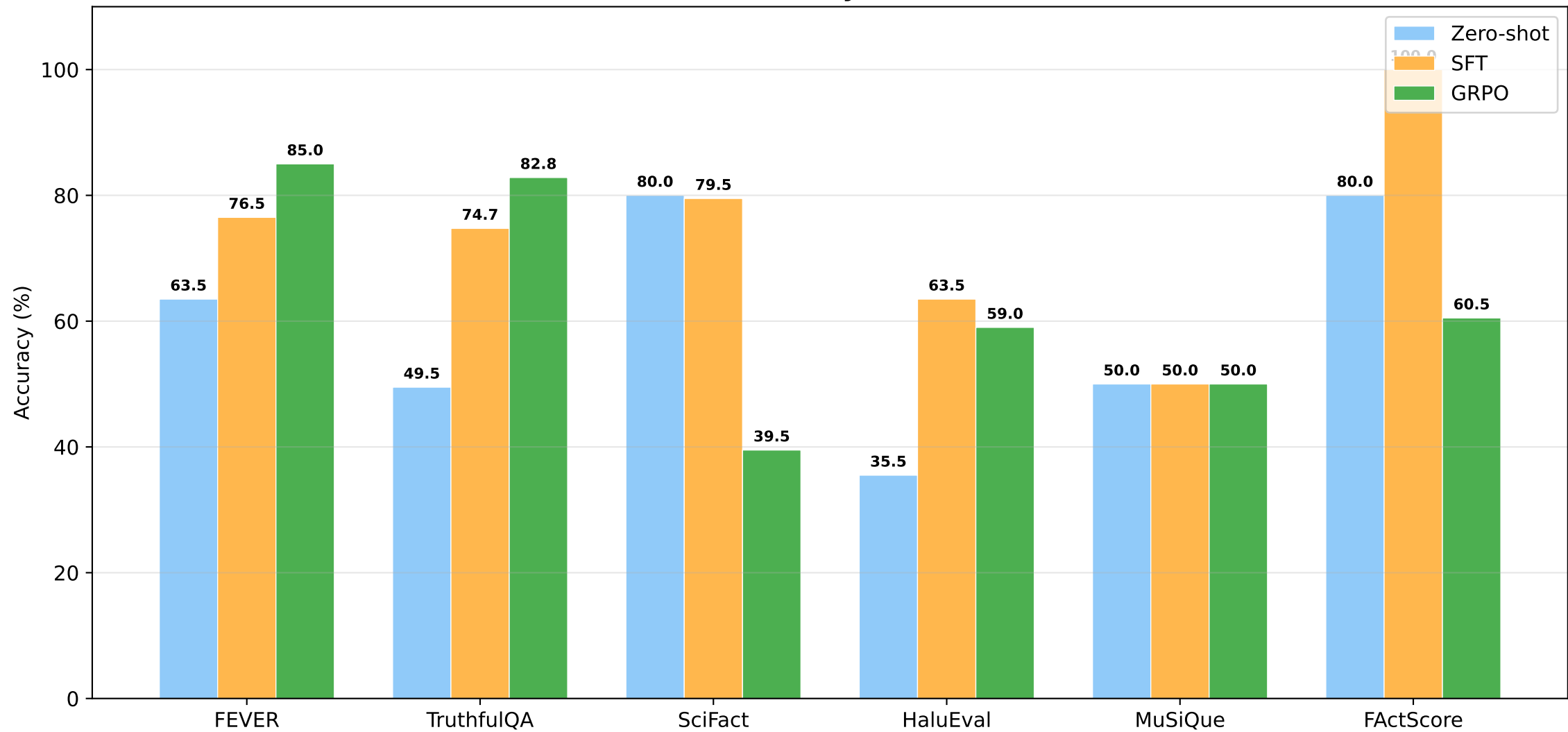
Fact Verification Accuracy Across 6 Benchmarks
