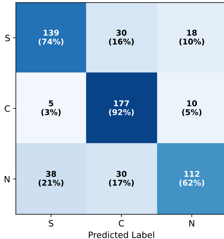
SFT (76.6%)
