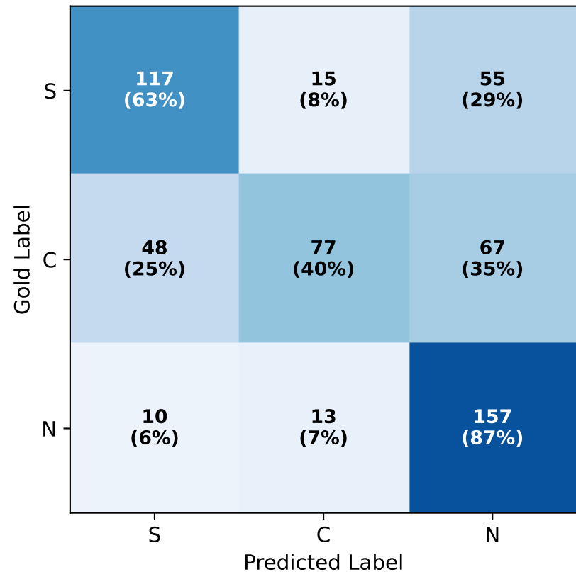
Zero-shot (62.8%)
