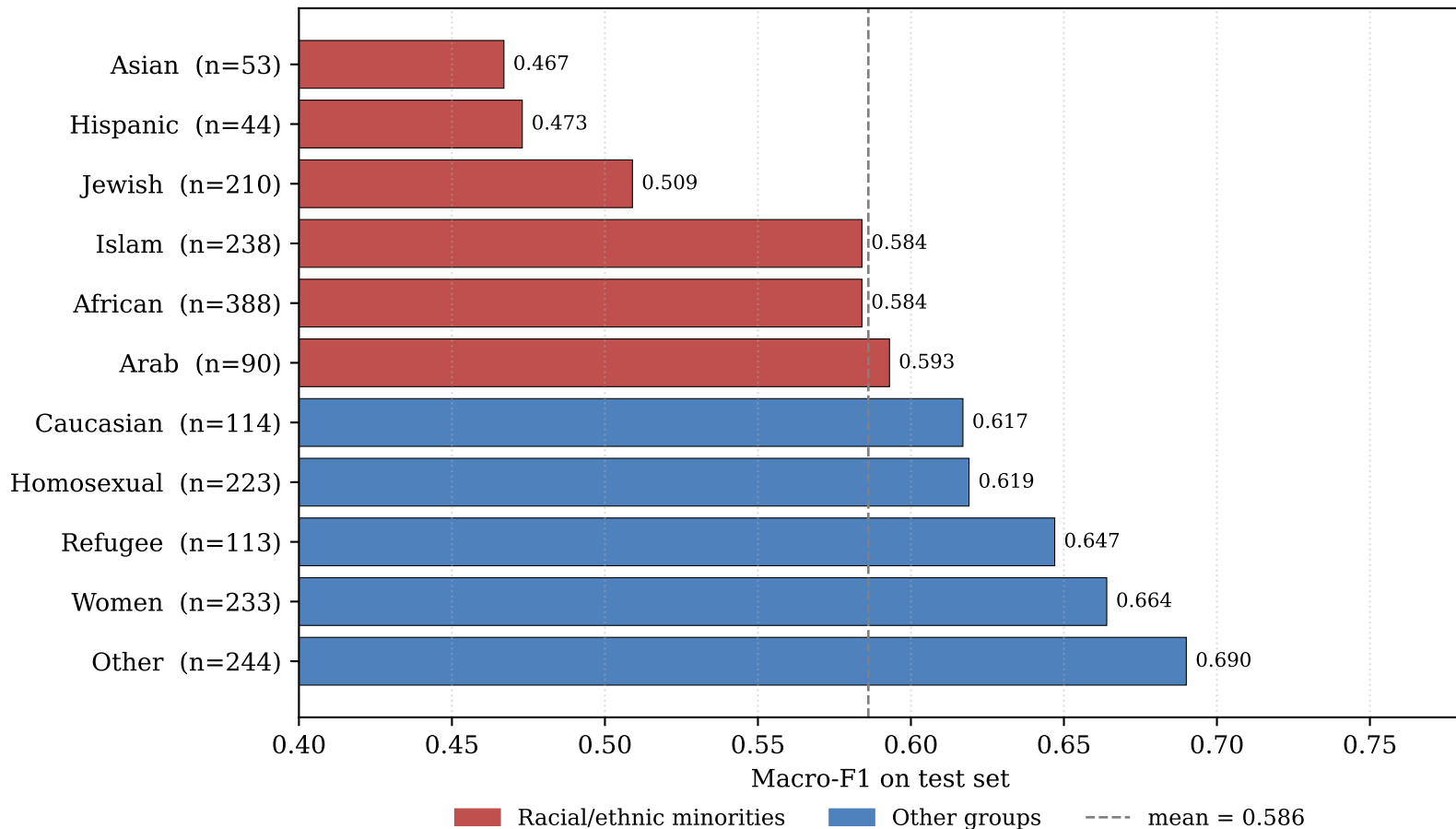
Per-target-group macro-F1 (final model, Exp 14)
