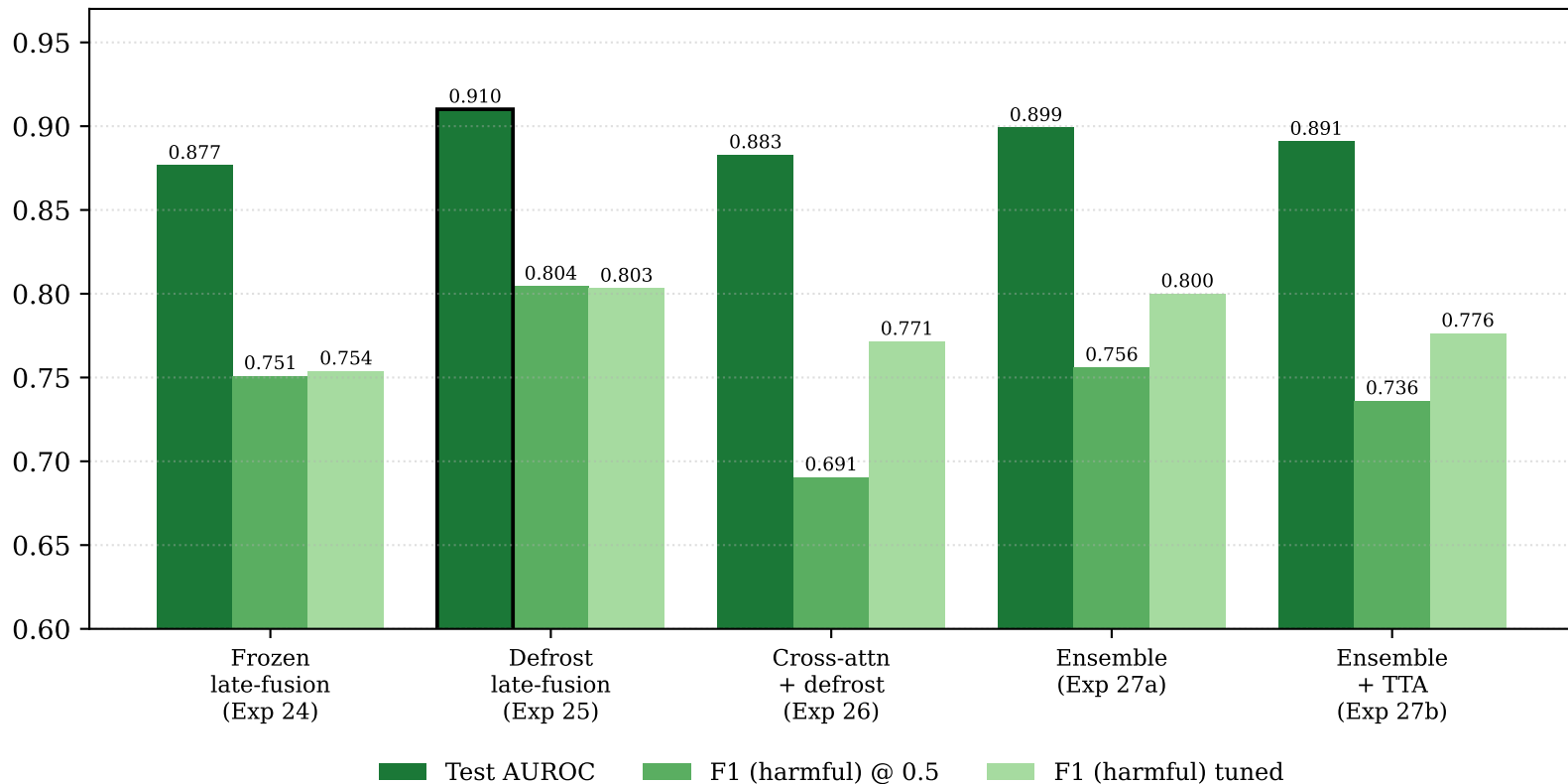
HarMeme: architecture comparison (Exp 24-27)
