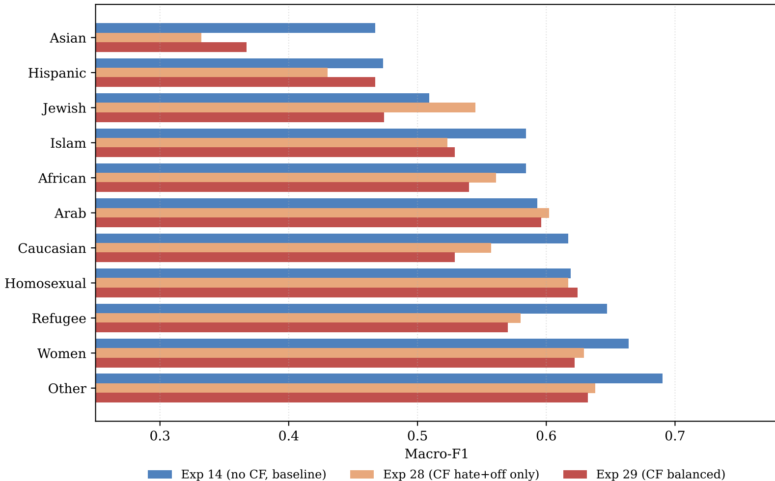
Counterfactual augmentation effect per target group
