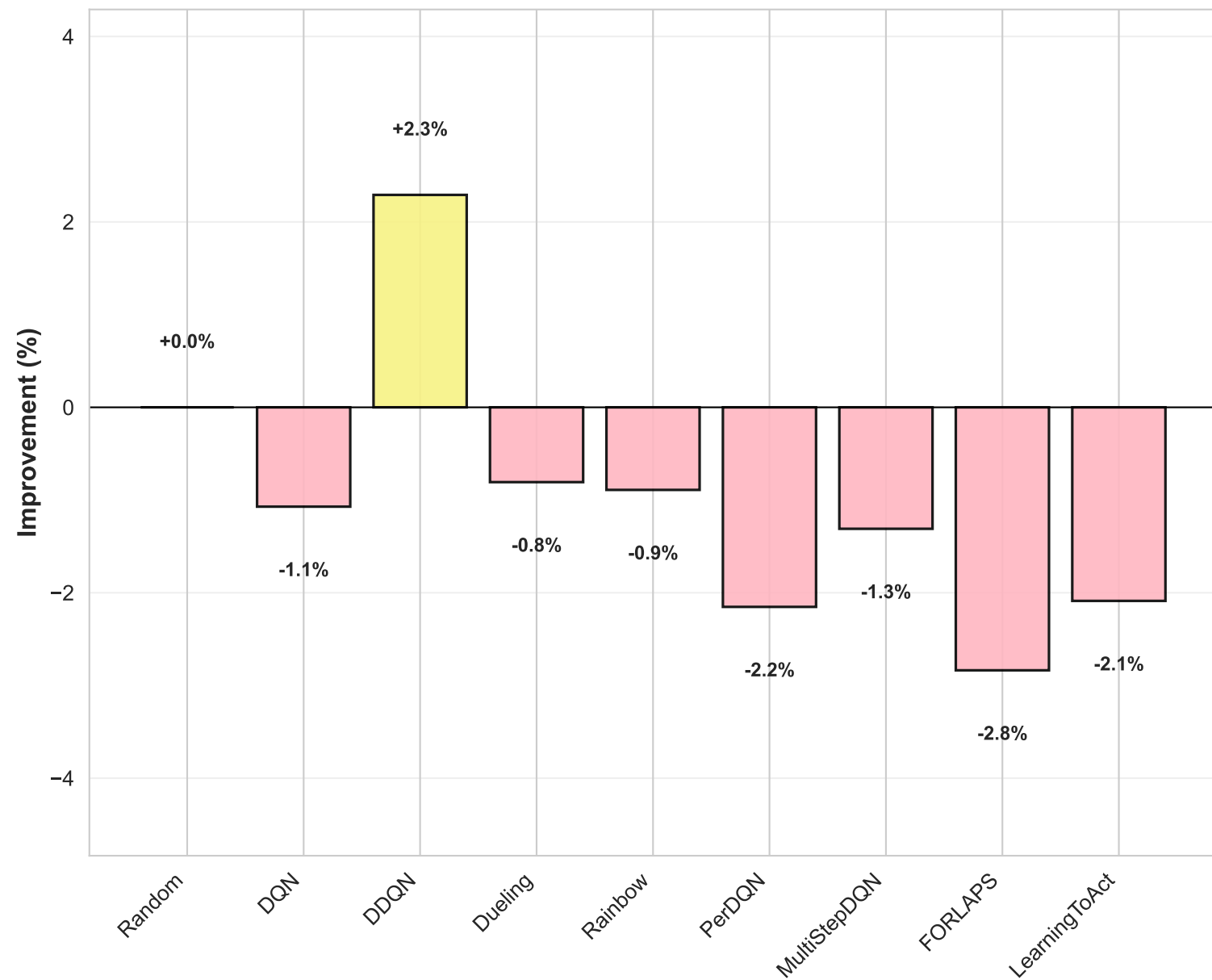
Idle Time Reduction (200 patients)
