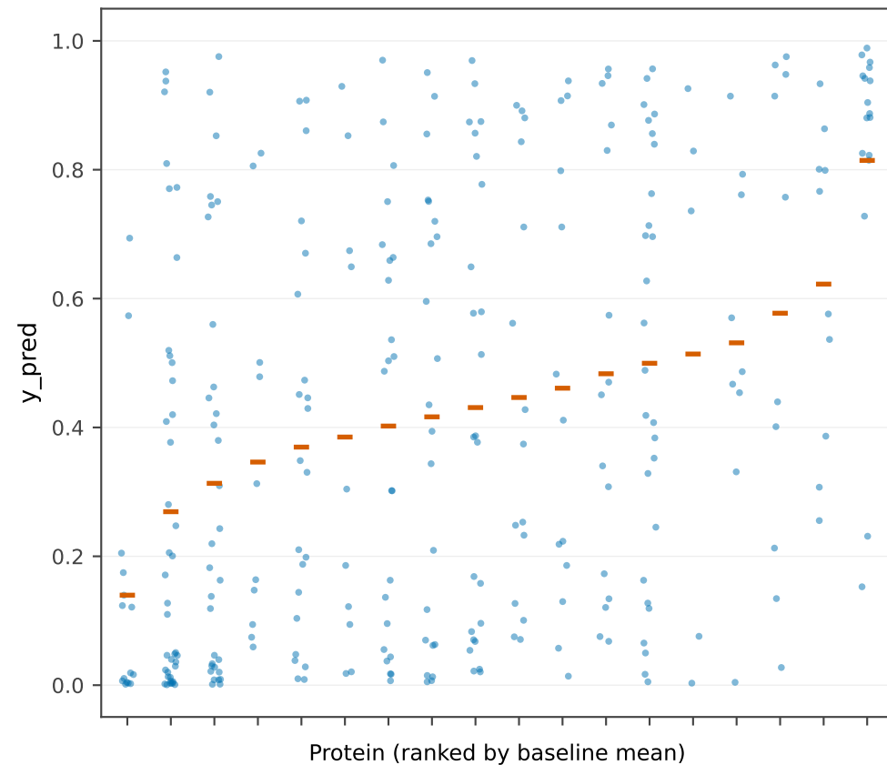
sequence only (ICC = 0.043)
