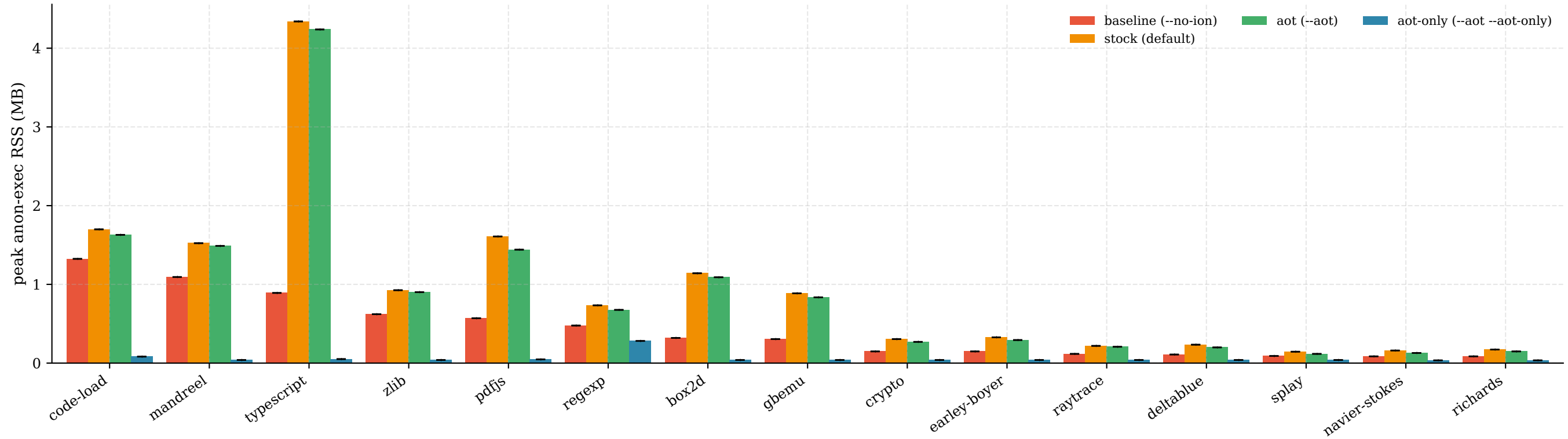
Per-process JIT code footprint across the Octane suite (N=1)
