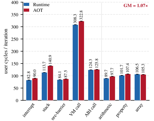
Figure 6: Preliminary User-mode cycles per iteration for runtime-generated and AOT Baseline code with Ion disabled (one fresh process per configuration). Labels give arithmetic means; whiskers show one standard deviation when multiple observations are available. The dotted rule separates five optimization-sensitive sites from three controls. GM is the geometric mean of the eight AOT/runtime ratios.
