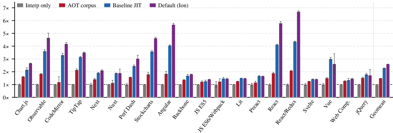
Speedup over interp only
