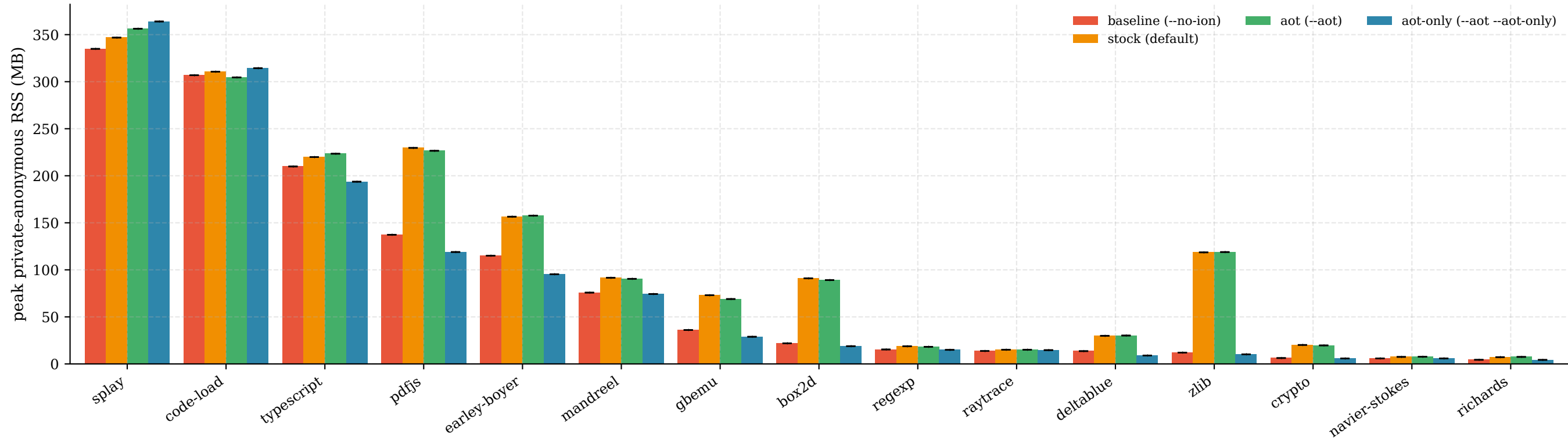
Per-process private anonymous RSS across the Octane suite (N=1)
