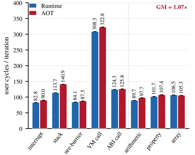
Figure 6: User-mode cycles per iteration for runtime-generated and AOT Baseline code with Ion disabled (ten fresh processes per configuration). Labels give arithmetic means; whiskers show one standard deviation when multiple observations are available. The dotted rule separates five optimization-sensitive sites from three controls. GM is the geometric mean of the eight AOT/runtime ratios.
