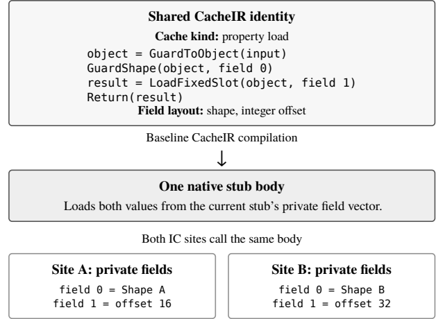
Figure 1: CacheIR separates a fast path’s structural identity from its site-specific values. The Baseline CacheIR compiler emits one native body for the shared program and field layout. Each IC site supplies a private field vector when it executes that body. Program syntax and values are schematic.
