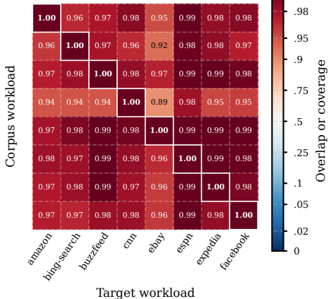
(c) Inline-cache stub-entry coverage
