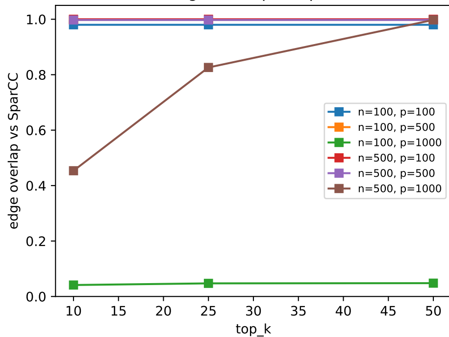
c edge overlap vs SparCC
