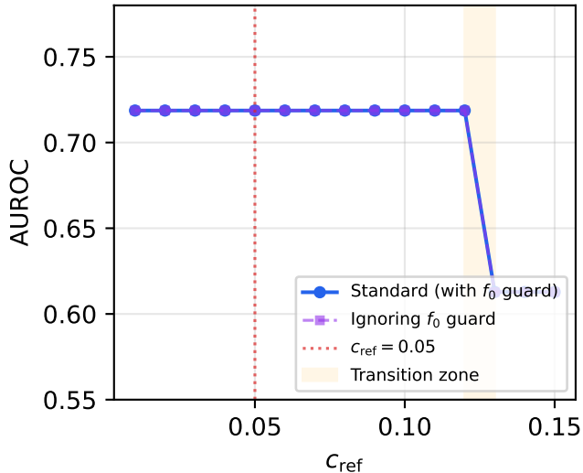
(a) v4 Simulator ( N = 500, P = 500 )
