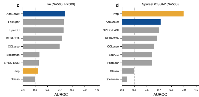
Figure 3 Cross-simulator comparison (9 methods). On v4 data (left), AdaCoNet dominates in the multinomial regime ( \alpha_0/p > c^* ). On SparseDOSSA2 Gaussian copula data (right), the Phase Transition Theorem downweights Spearman ( w_S = 0.083 due to f_0 = 0.66 ), achieving AUROC 0.714 – second only to standalone proportionality (0.899).
