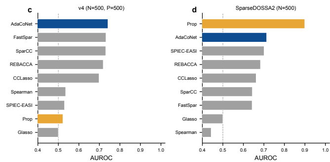
Figure 3 Cross-simulator comparison (9 methods). On v4 data (left), AdaCoNet dominates in the multinomial regime ( \alpha_0/p > c^* ). On SparseDOSSA2 Gaussian copula data (right), the MSE Reliability Bound downweights Spearman ( w_S = 0.083 due to f_0 = 0.66 ), achieving AUROC 0.714 – second only to standalone proportionality (0.899).
