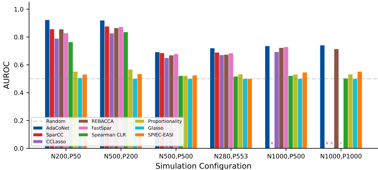
a | Accuracy Across Configurations (9 Methods)
