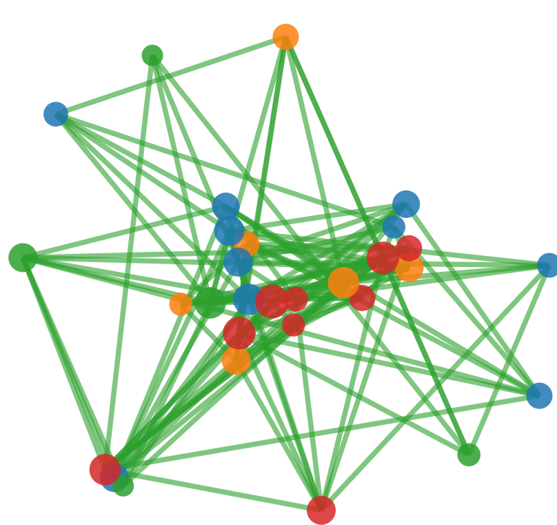
AdaCoNet Nodes=30 Edges=121 Density=0.278 Mod=0.225
