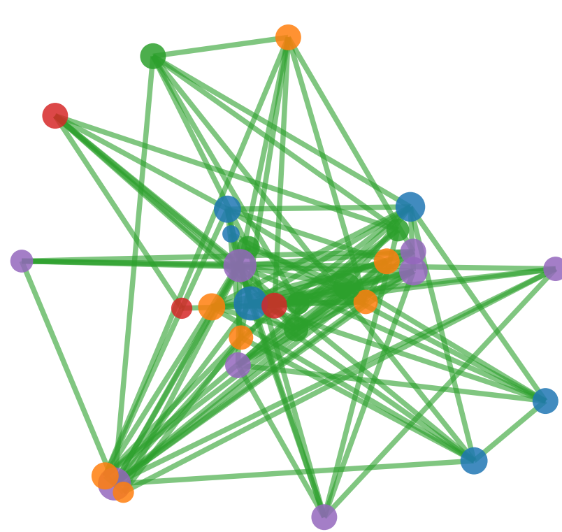
SparCC Nodes=30 Edges=108 Density=0.248 Mod=0.226
