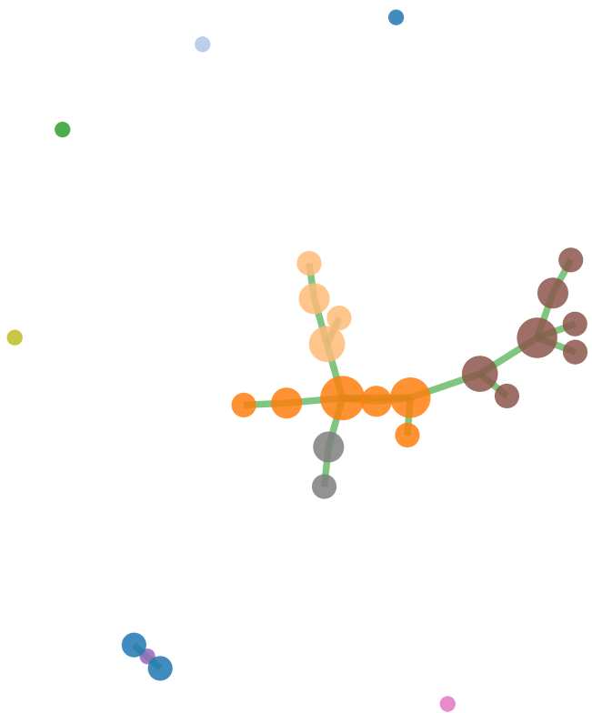
Ground Truth Nodes=30 Edges=20 Density=0.046 Mod=0.565
