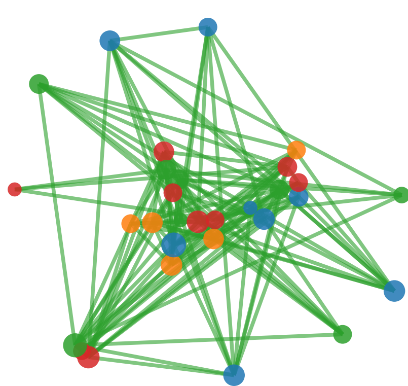
SPIEC-EASI Nodes=30 Edges=121 Density=0.278 Mod=0.204
