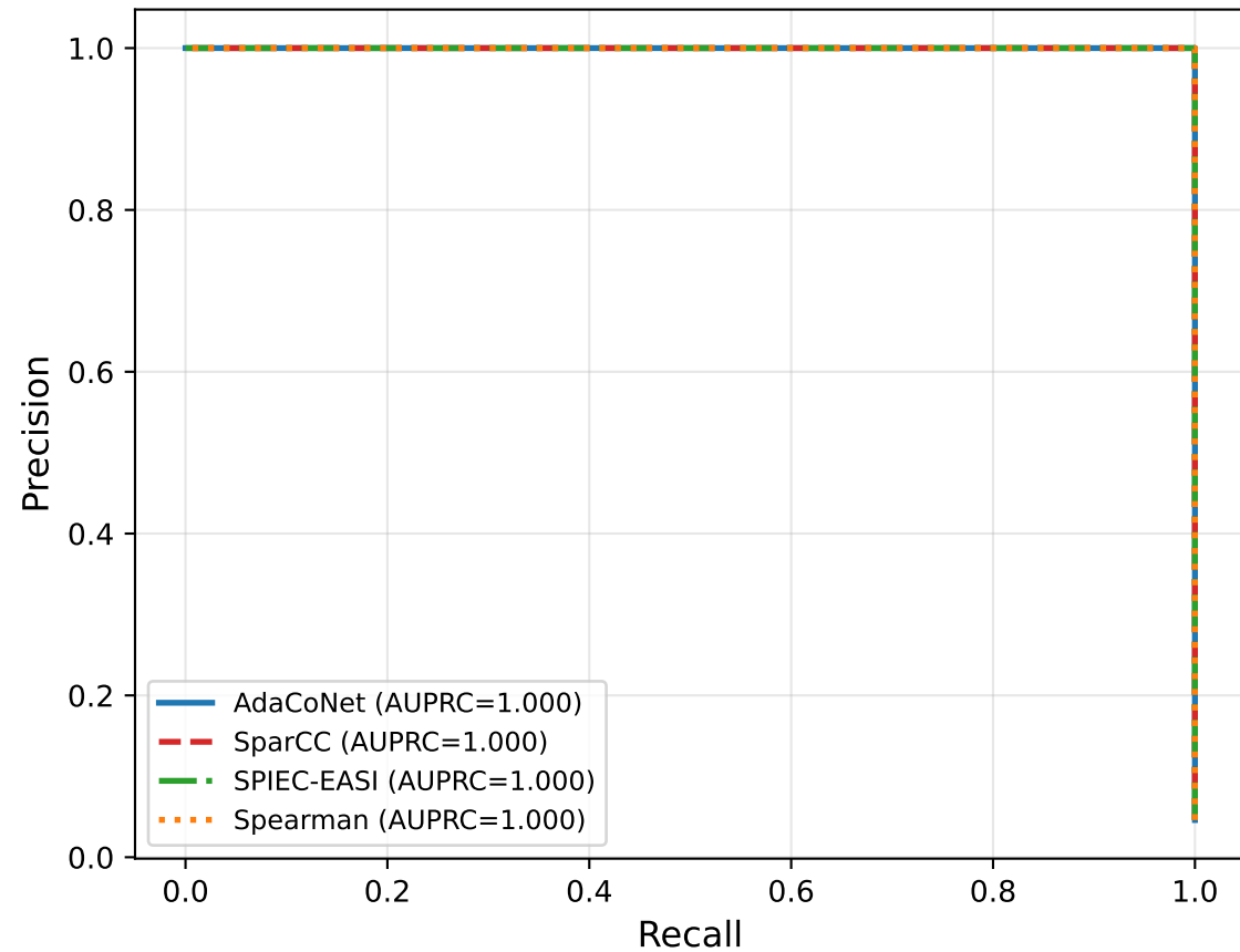
Precision-Recall Curve
