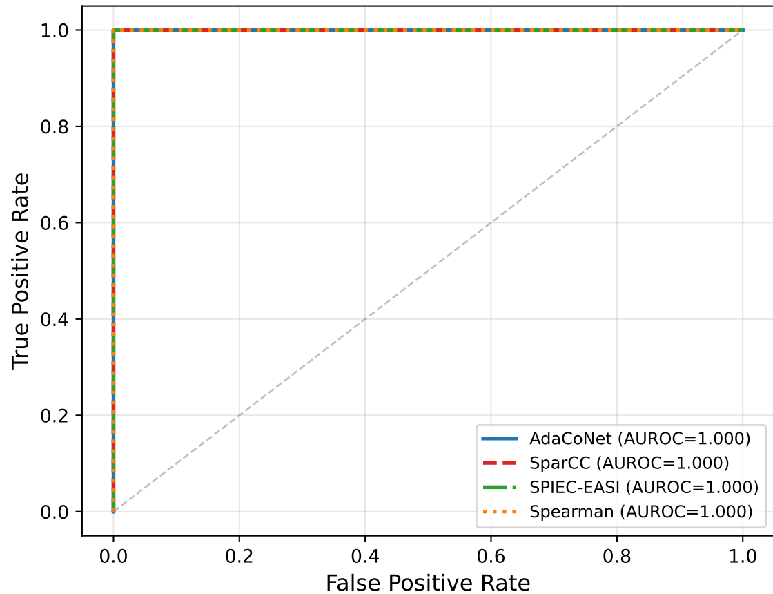
ROC Curve
