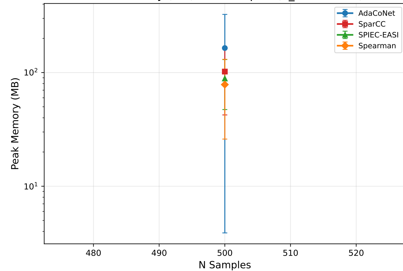
Peak Memory (MB) vs n samples (n_taxa=1000)
