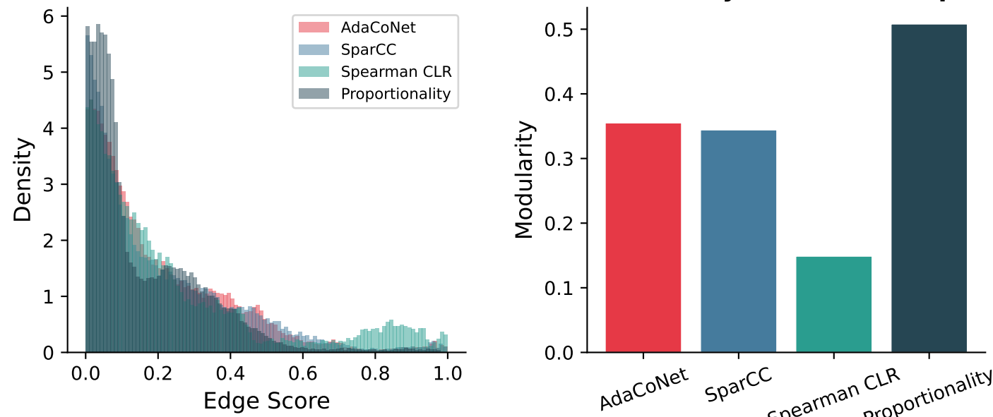
Score Distribution (Real Data) Network Modularity (Real Data, top 5% edges)
