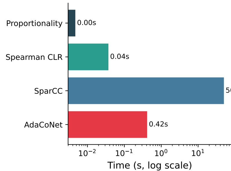
Runtime on Real Data (N=697, P=361)
