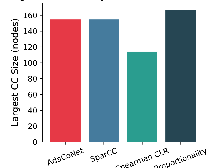
Largest Connected Component Size (Real Data)
