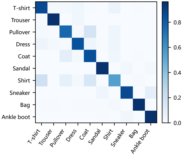
FashionMNIST 混淆矩阵
