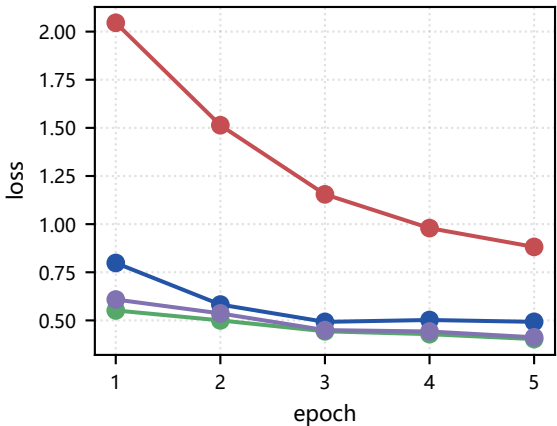
FashionMNIST 测试损失
