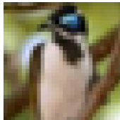
T:bird P:dog 0.98
