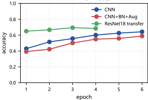
CIFAR-10 验证轨迹
